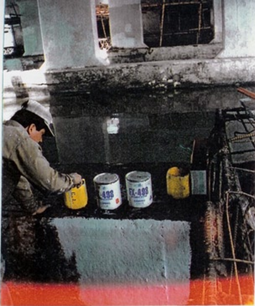
FX-498 Hydro-Ester®, 100% Solids, Water Insensitive Coating is being applied at the water line by brush.
