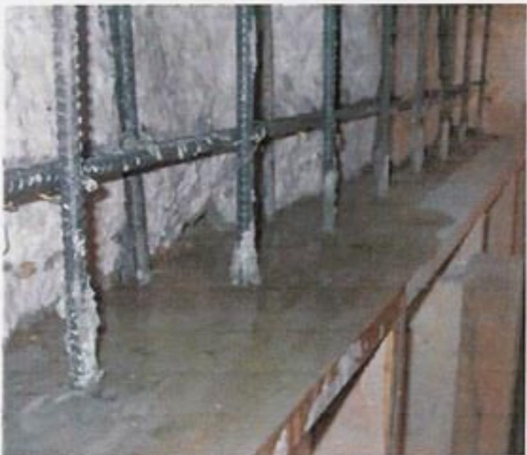
Walls and ceiling are rebuilt using FX-792 Epoxy Bonding Agent, FX-228 Non-Shrink Non-Metallic Grout, and FX-253 Trowel Grade Mortar.
