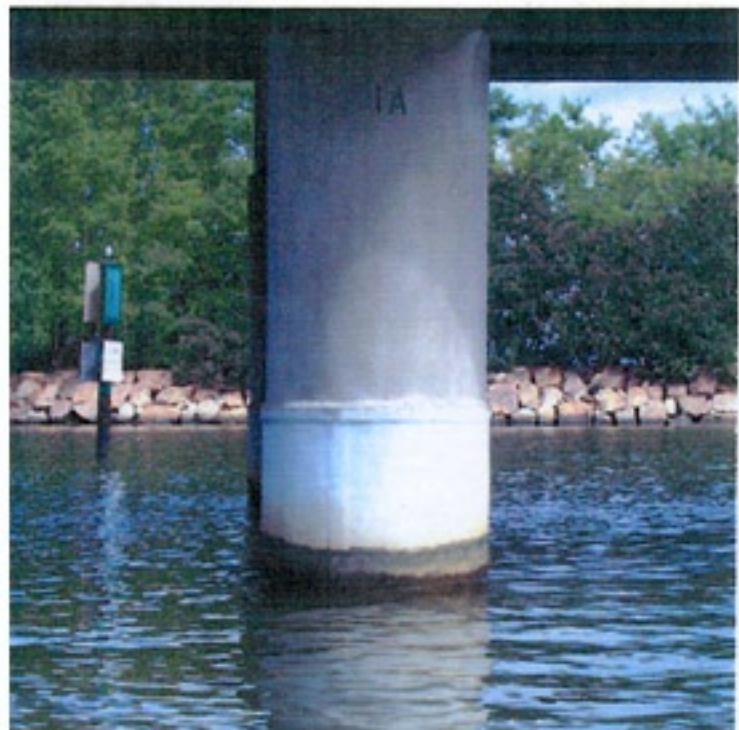
Close up view showing FX-70® System in excellent condition after 20+ years of service.
